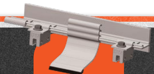
S-5! Colorgard® with S-5-N 1.5 Clamp
